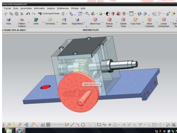
Fig (3): Final Assembly of Attachment for Gear Cutting FABRICATION ATTACHMENT TO LATHE:
