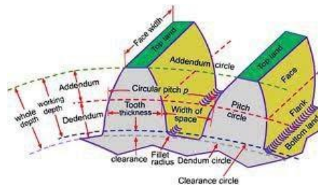
Fig (2): Spur Gear Nomenclature
