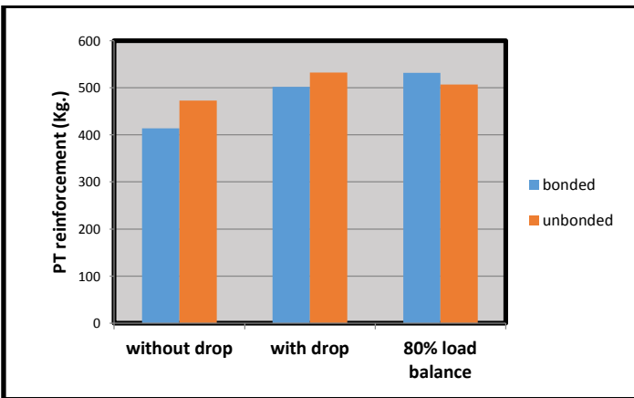
Fig :26 PT Reinforcement of bonded/unbonded for double span for 9 Mt. length of span
