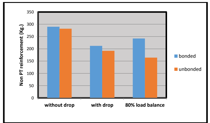
Fig : 28 Non PT Reinforcement of bonded/unbonded for triple span for 8 Mt. length of span
