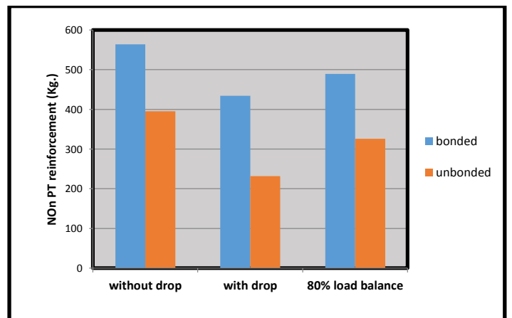
Fig : 29 Non PT Reinforcement of bonded/unbonded for triple span for 8 Mt. length of span
