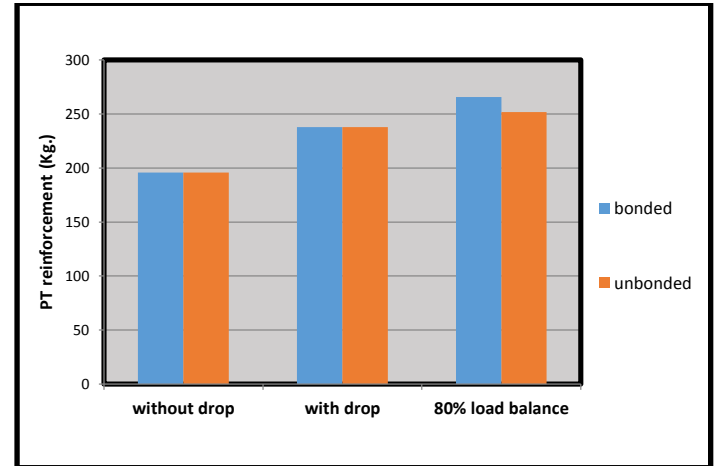
Fig : 22 PT Reinforcement of bonded/unbonded for single span for 8 Mt. length of span
