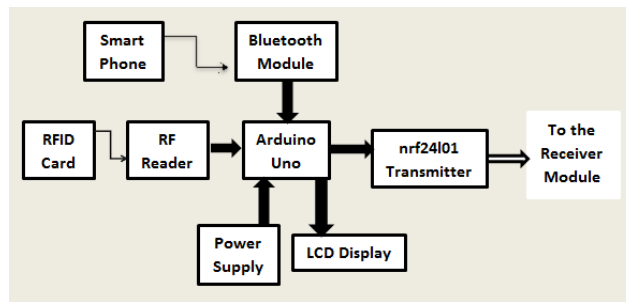
Figure 1: Block diagram of trolley system
