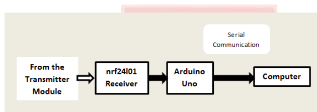
Figure 2: Block diagram of receiver side.
