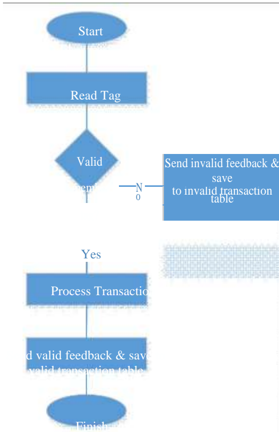
Figure 4: Simulation For Attendance Management Rules
