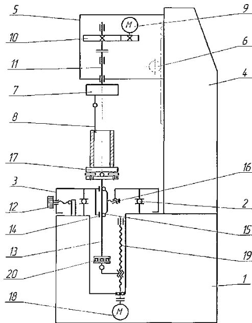
Fig. 1. Kinematic diagram of modernized BE-20A roundness gauge
