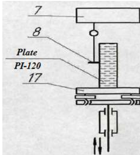
Fig. 2. Scheme of checking the error of axial displacement
