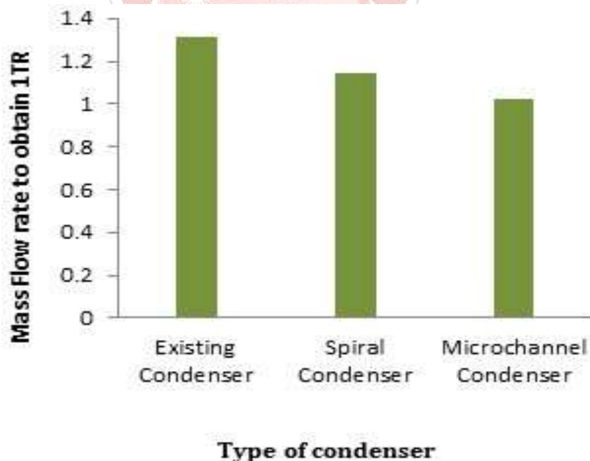
Fig. 6 Type of condenser recommended in to operation vs. Mass Flow rate to achieve 1TR
