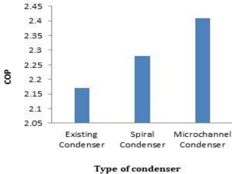
Fig. 5 Effect studied between type of condenser and respective COP obtained
