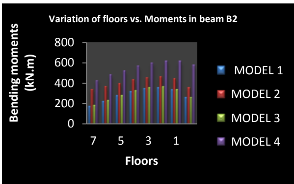
Fig. 1: Bending moment comparison of beam B2 for earthquake loading
